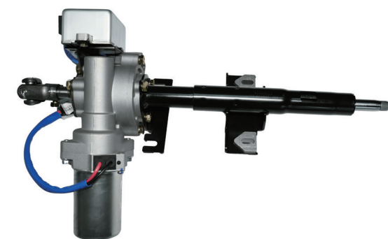
Electrical Power Steering Column(EPS) 电子助力转向管柱
